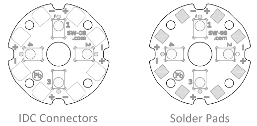
PCB Markings 1:1
